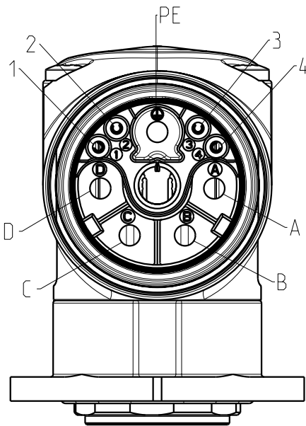
plug face male
