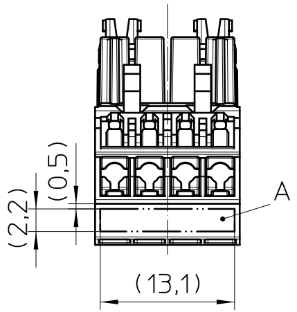
view X
