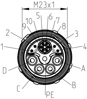
plug face male
