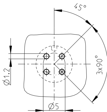
PCB-Layout (advice)
