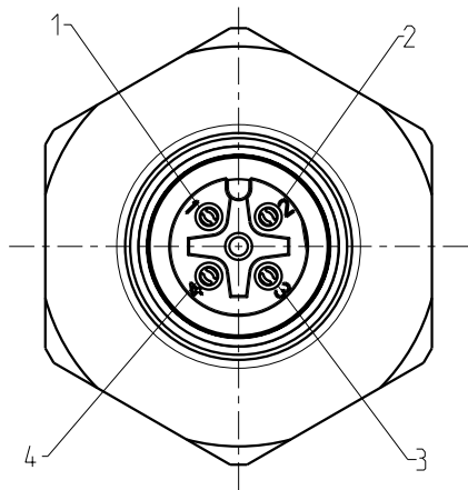
View of pin assignment Plug-in side
