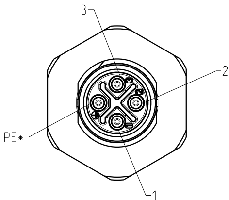
View of pin assignment Plug-in side
