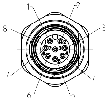
View of pin assignment Plug-in side
