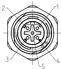
View of pin assignment Plug-in side
