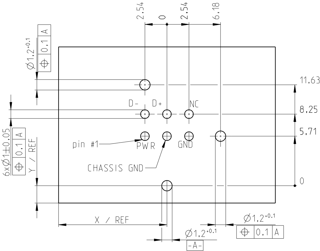
pin assignment with view of the component side of the pin insert
