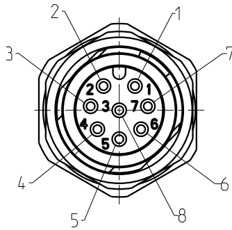
View of pin assignment Plug-in side
