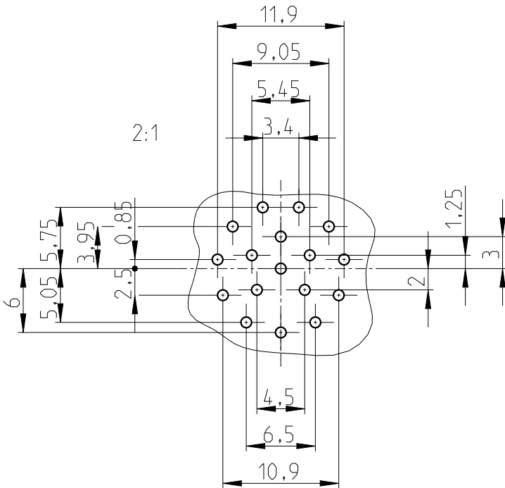
PCB-layout (advice)
