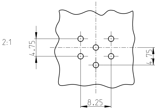
PCB-Layout (advice)
