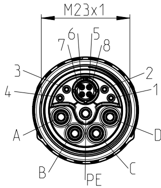
socket face female
