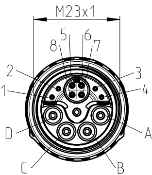
plug face male
