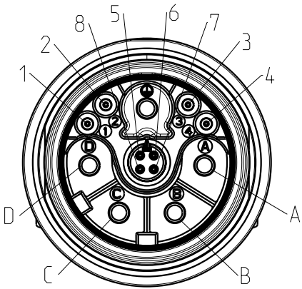
plug face male
