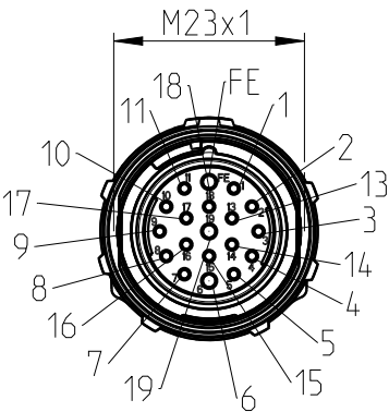
plug face male
