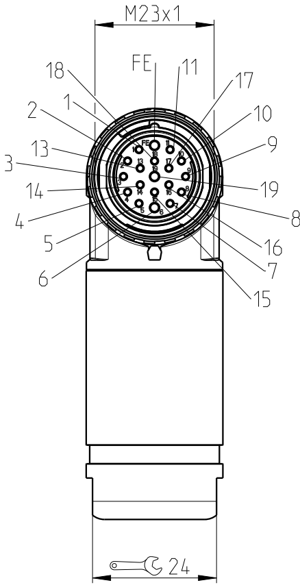
socket face female
