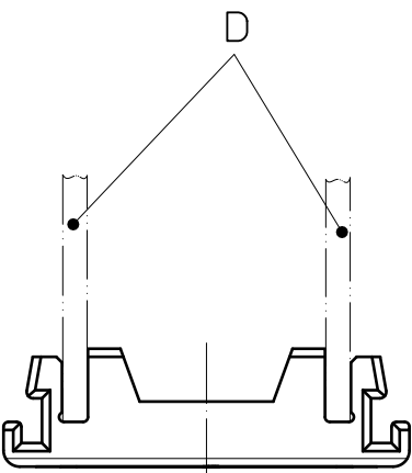
Assembly example
