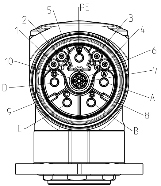
plug face male
