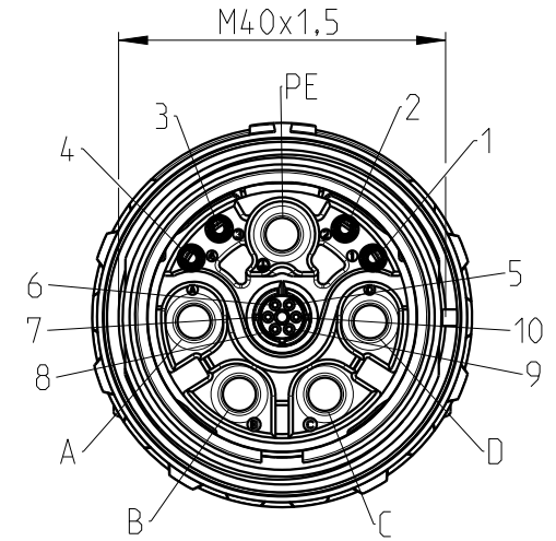
socket face female
