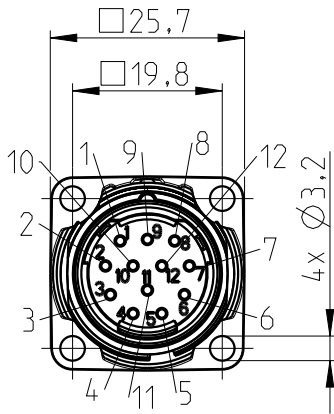
socket face female
