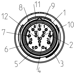
socket face female
