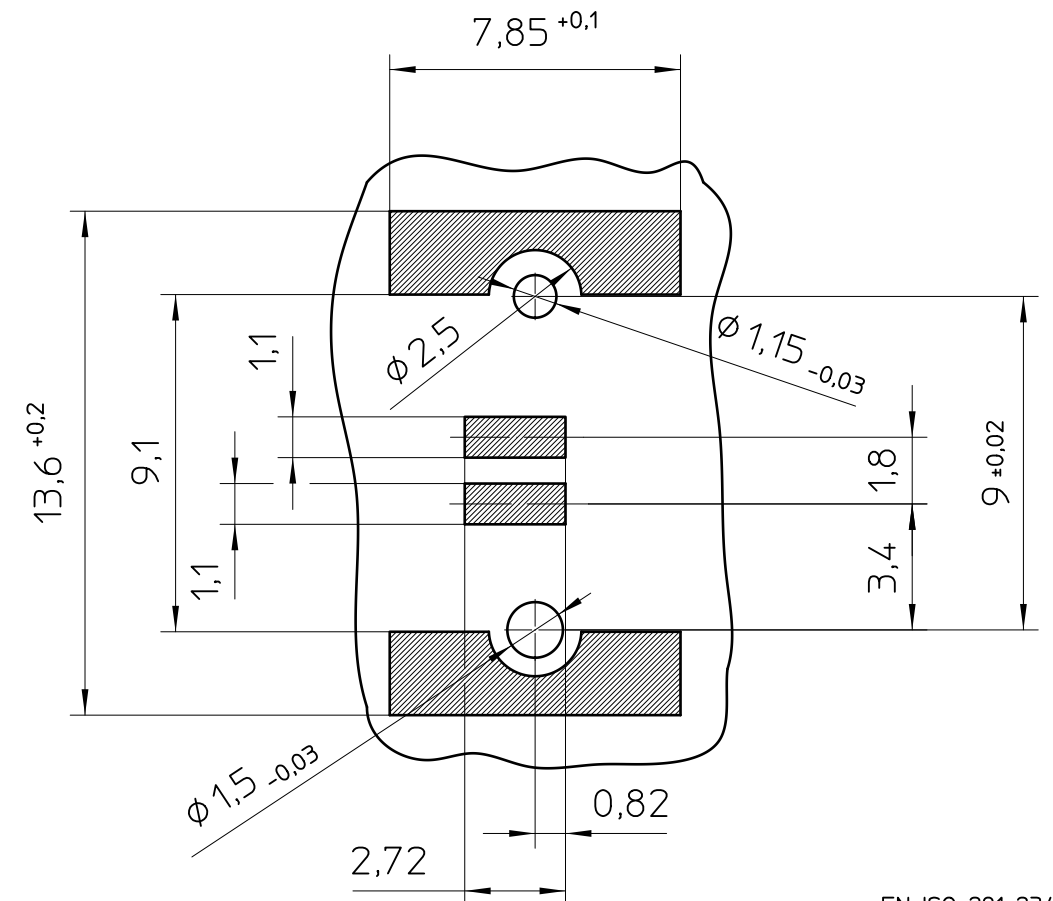
Pinning reccomendation
