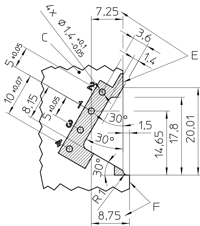
Recommended Main PCB
