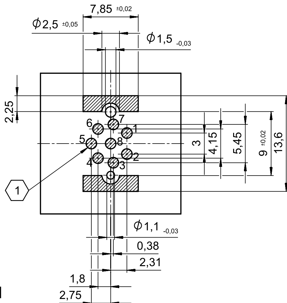
PCB-layout (advice)
