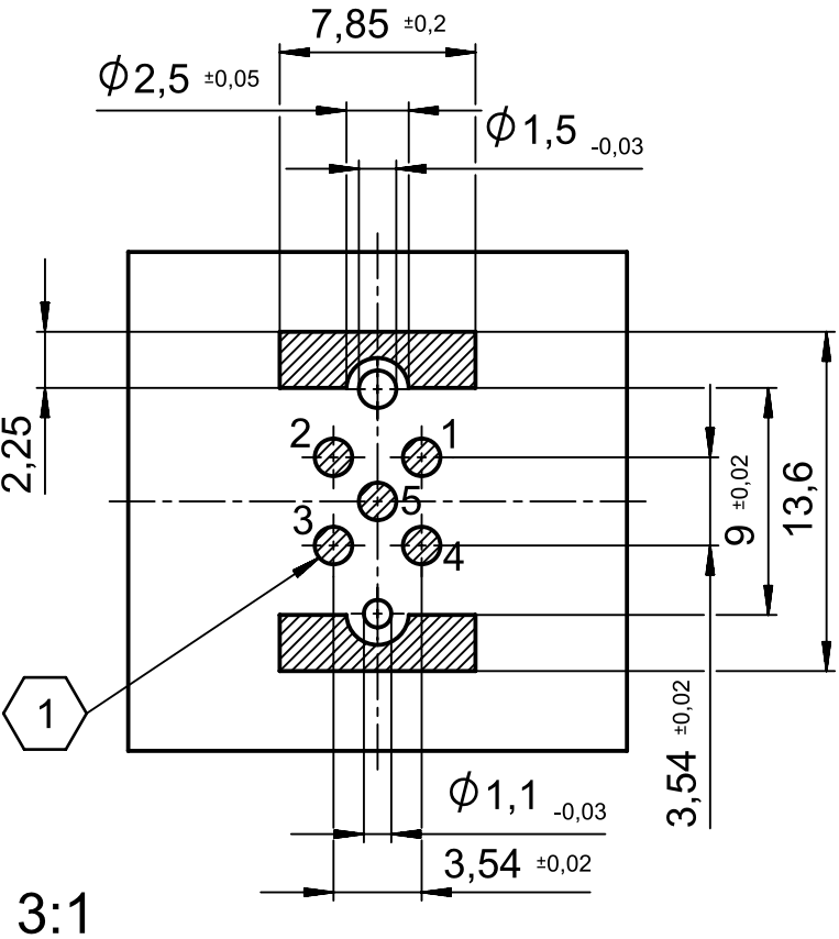
PCB-layout (advice)
