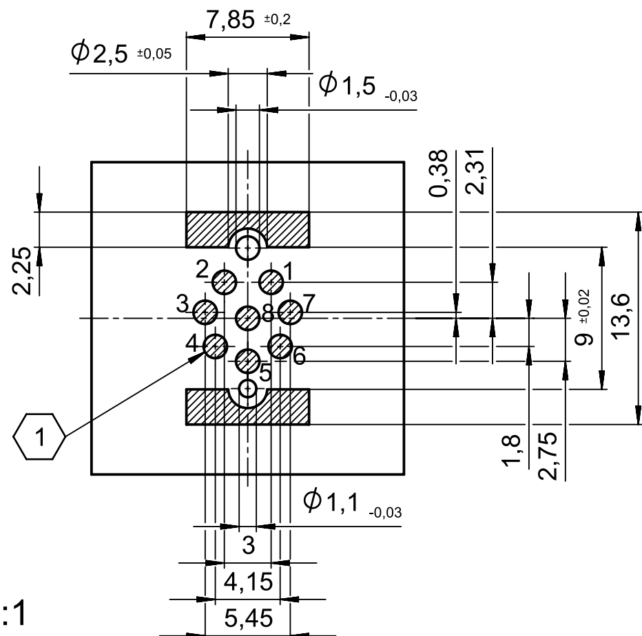
PCB-layout (advice)
