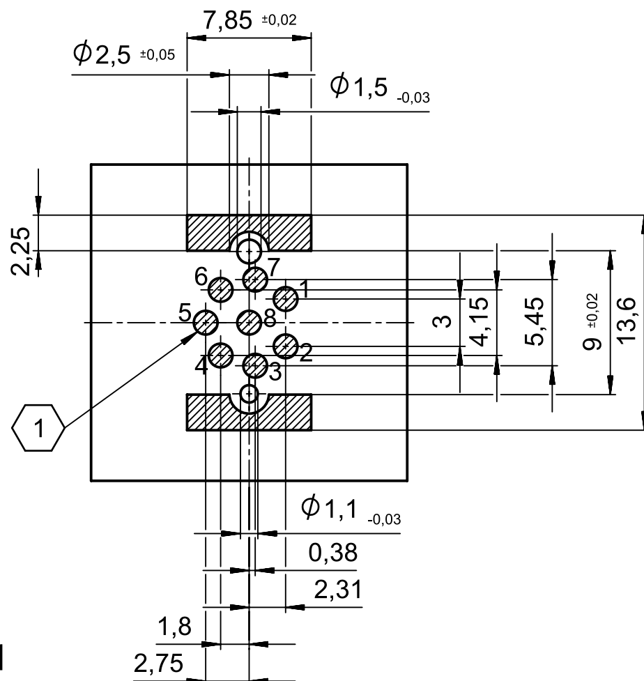
PCB-layout (advice)
