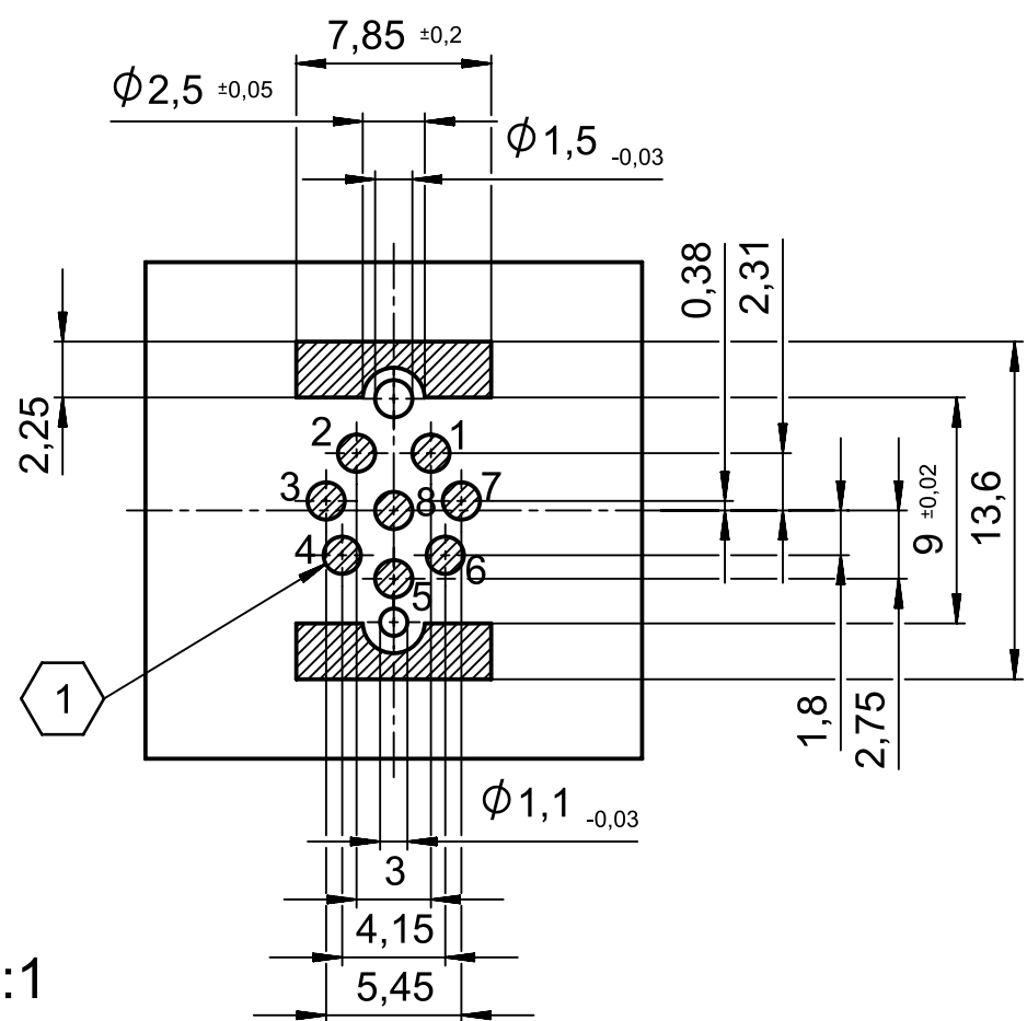
PCB-layout (advice)
