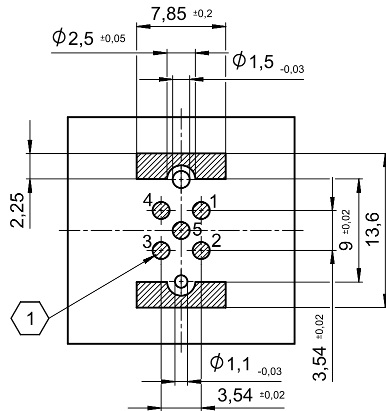
PCB-layout (advice)
