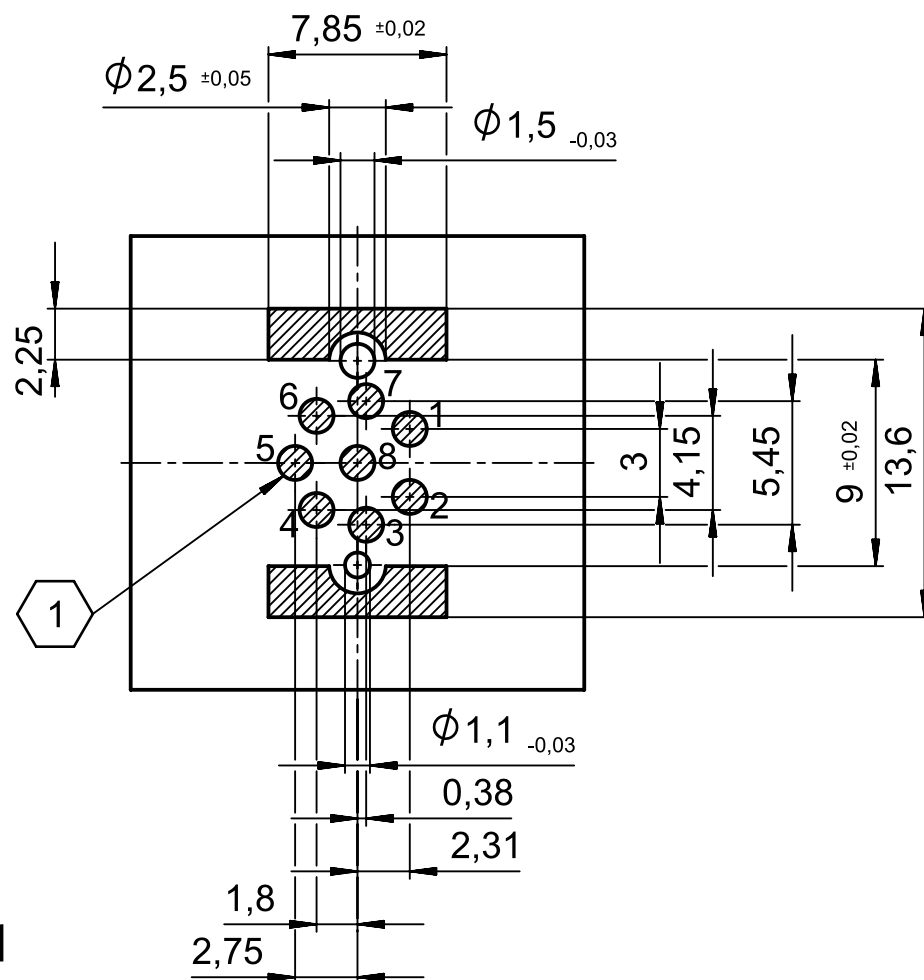
PCB-layout (advice)
