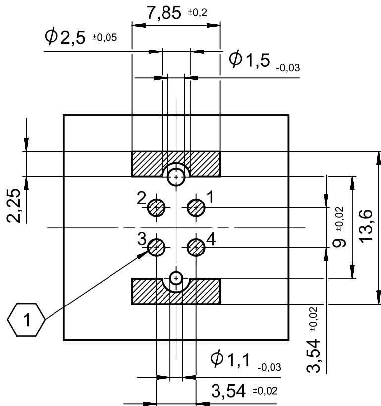
PCB-layout (advice)
