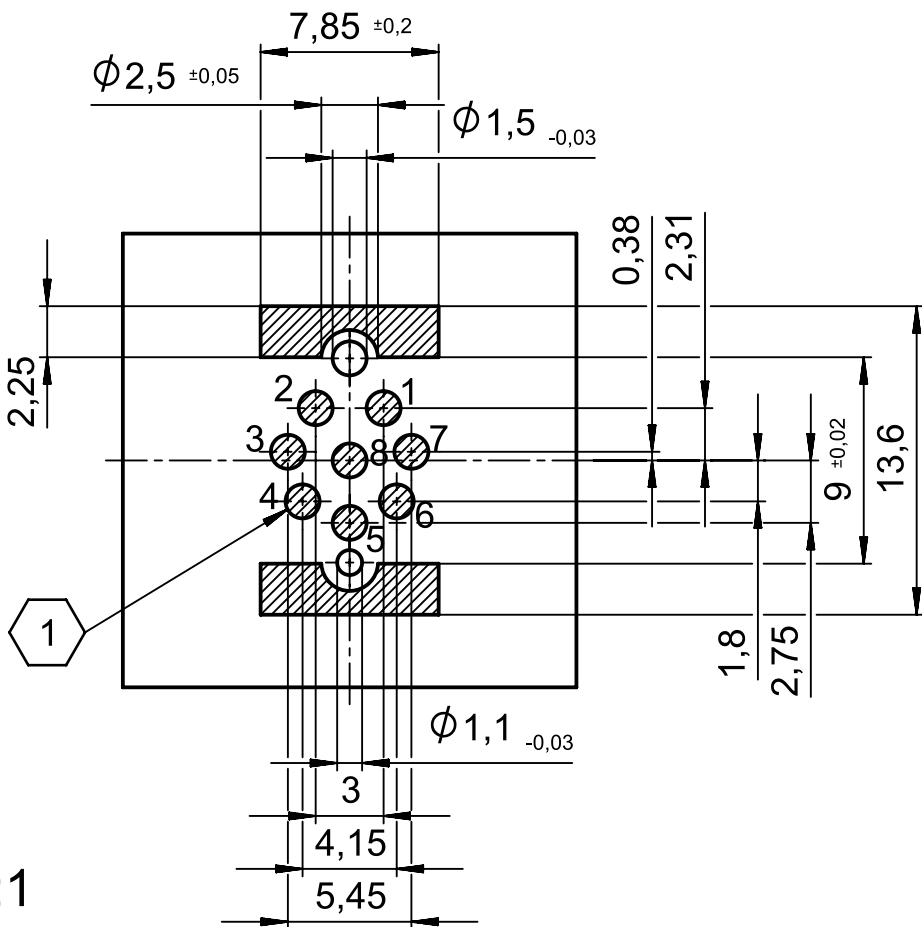
PCB-layout (advice)
