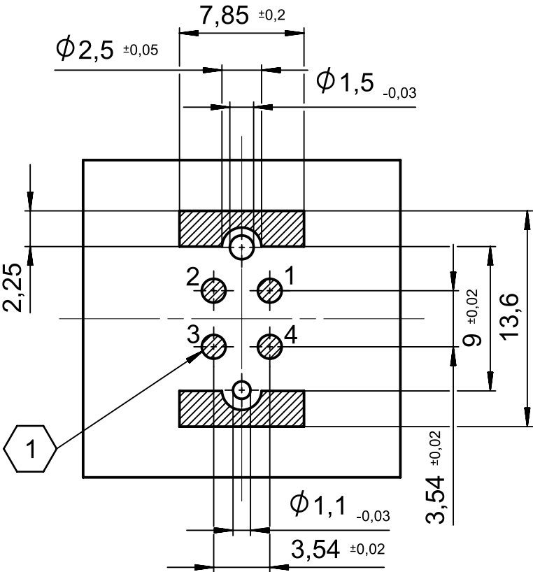
PCB-layout (advice)
