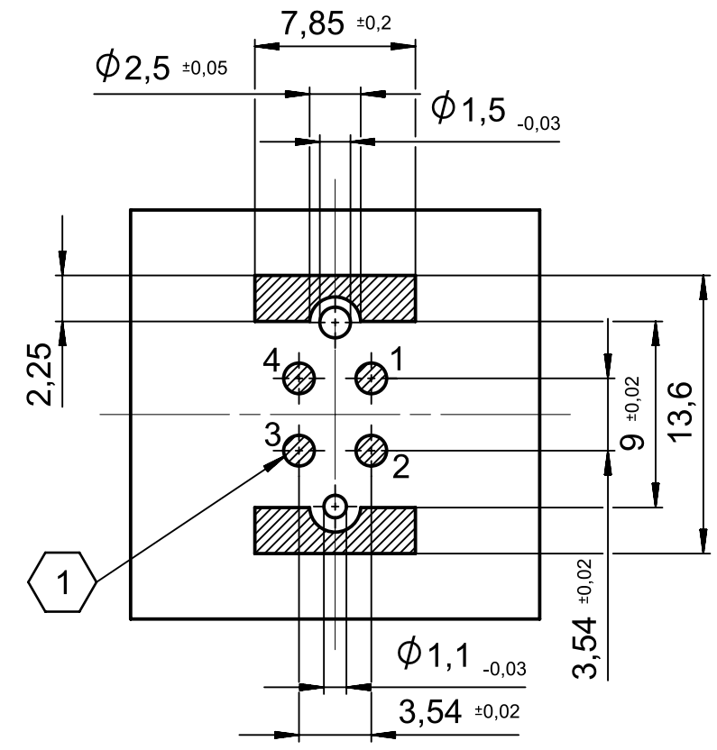
PCB-layout (advice)
