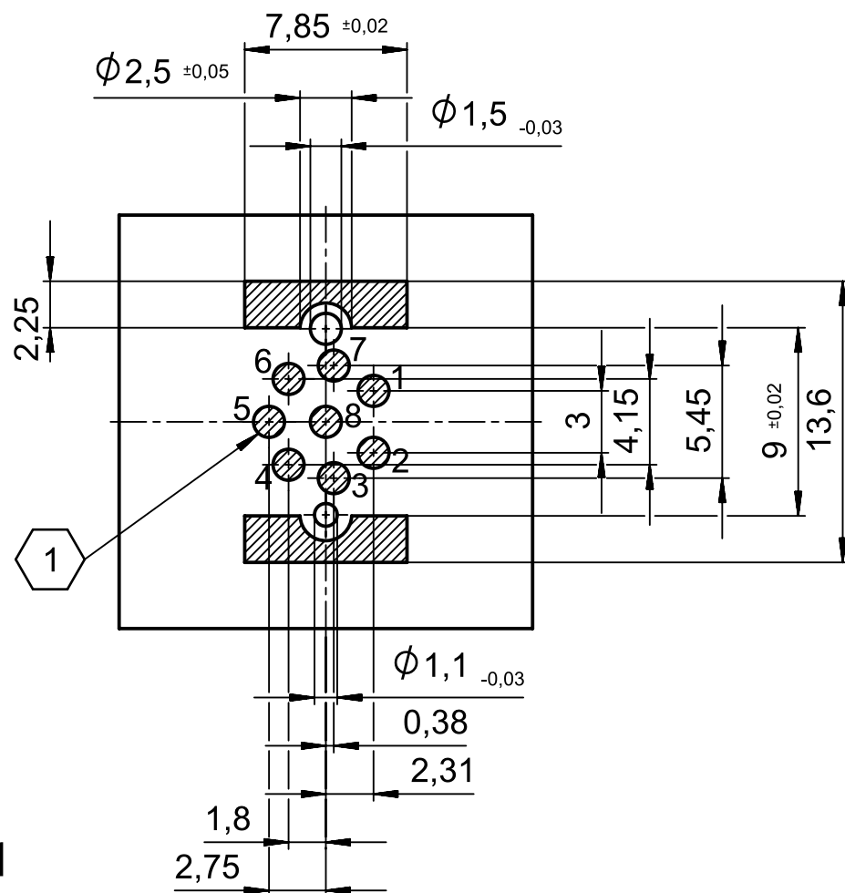
PCB-layout (advice)
