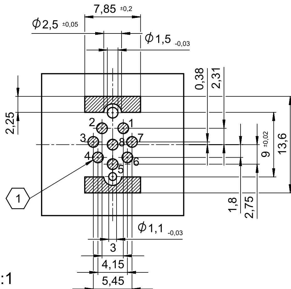
PCB-layout (advice)
