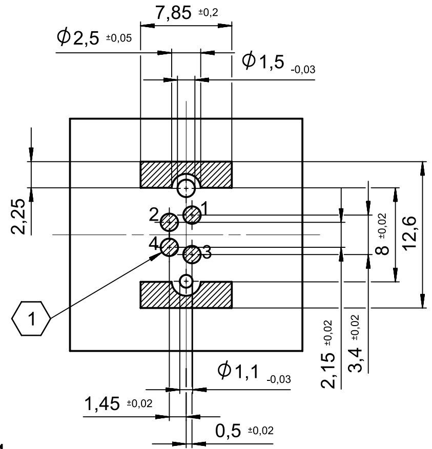
PCB-layout (advice)
