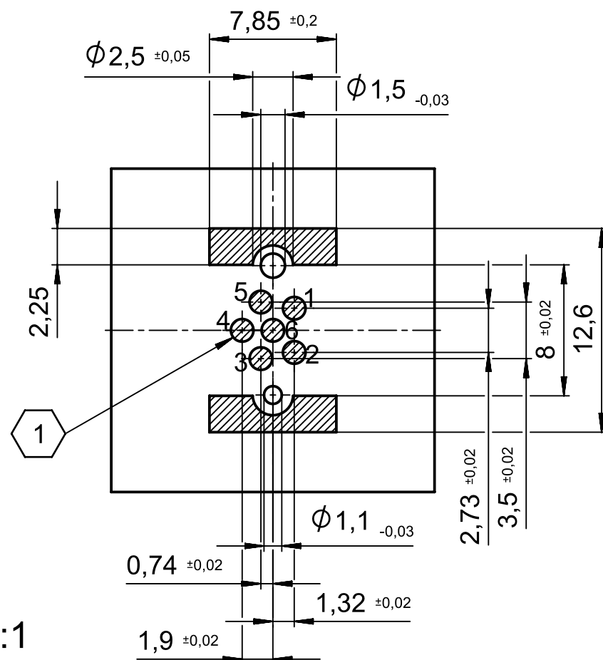
PCB-layout (advice)
