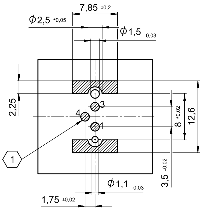
PCB-layout (advice)
