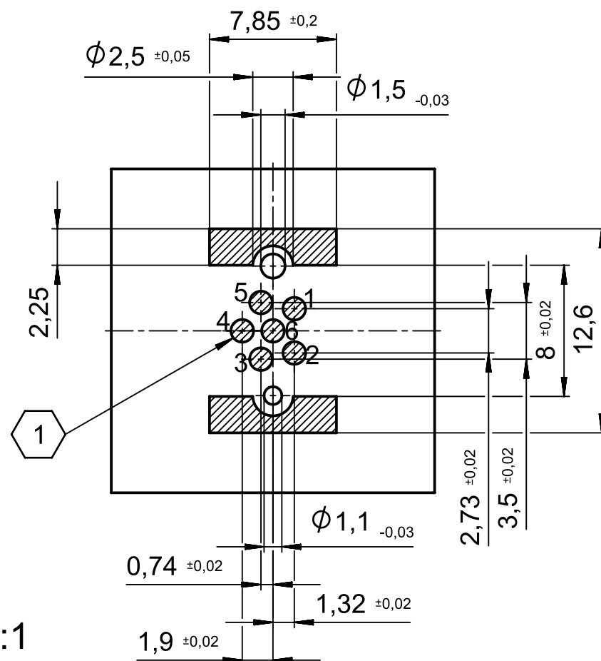
PCB-layout (advice)
