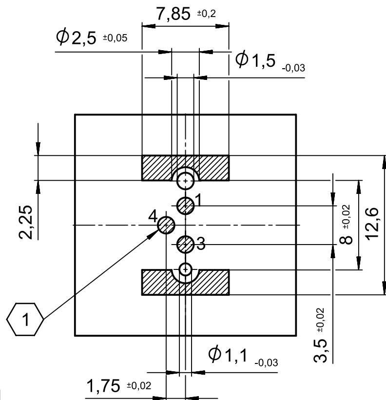
PCB-layout (advice)
