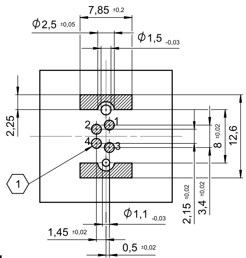
PCB-layout (advice)
