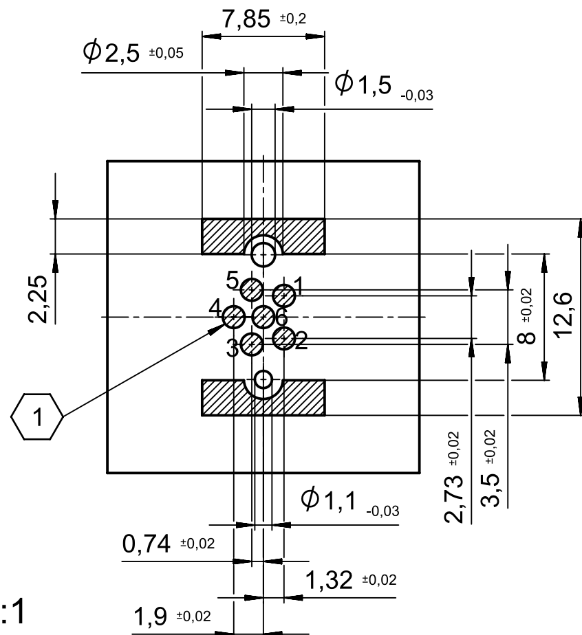
PCB-layout (advice)
