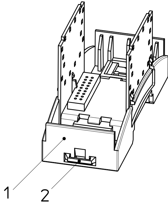
HOUSING LOWER PART with FOOT CATCH mounted
