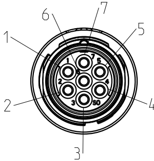
socket face female
