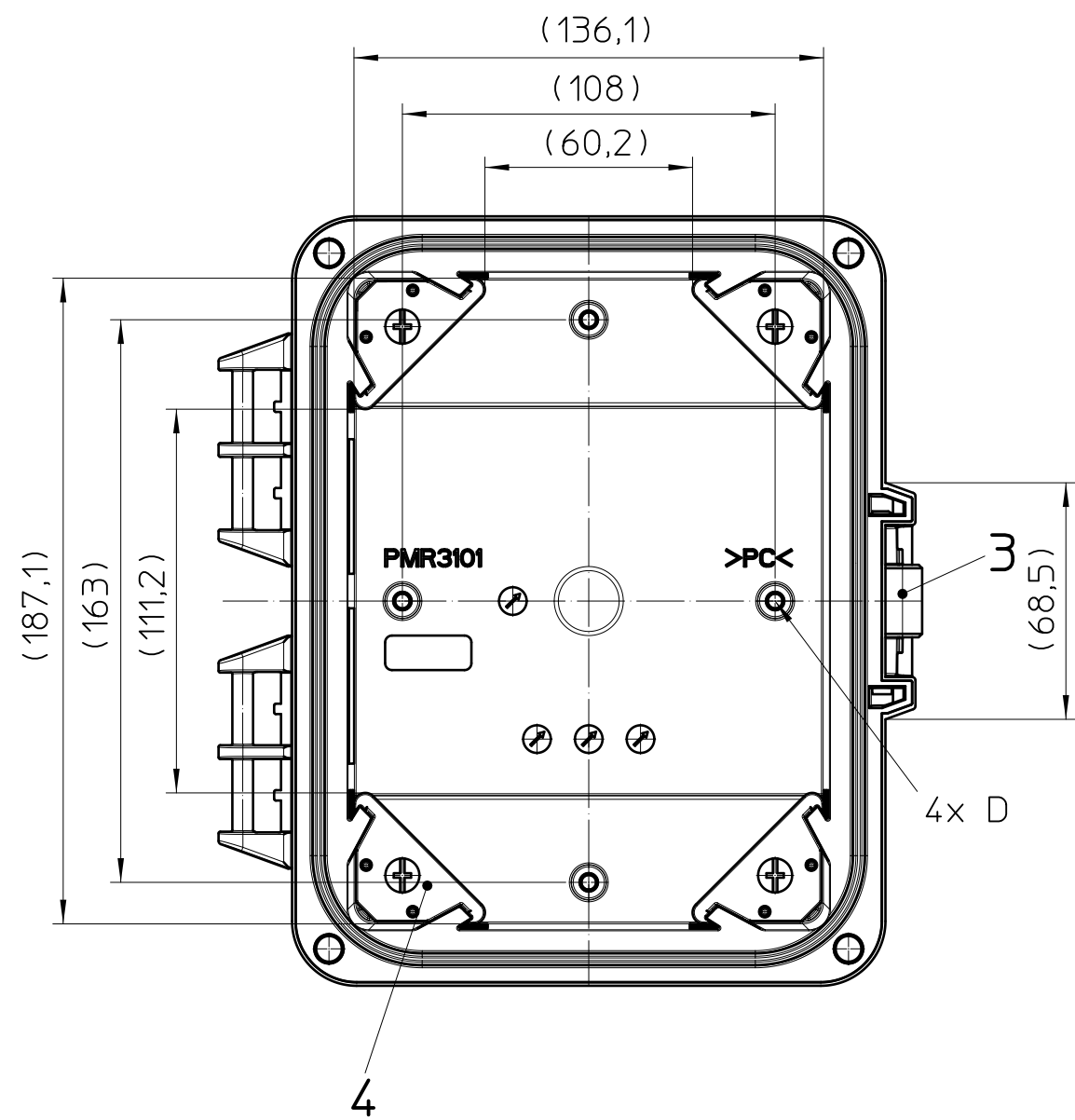
Front view without cover
