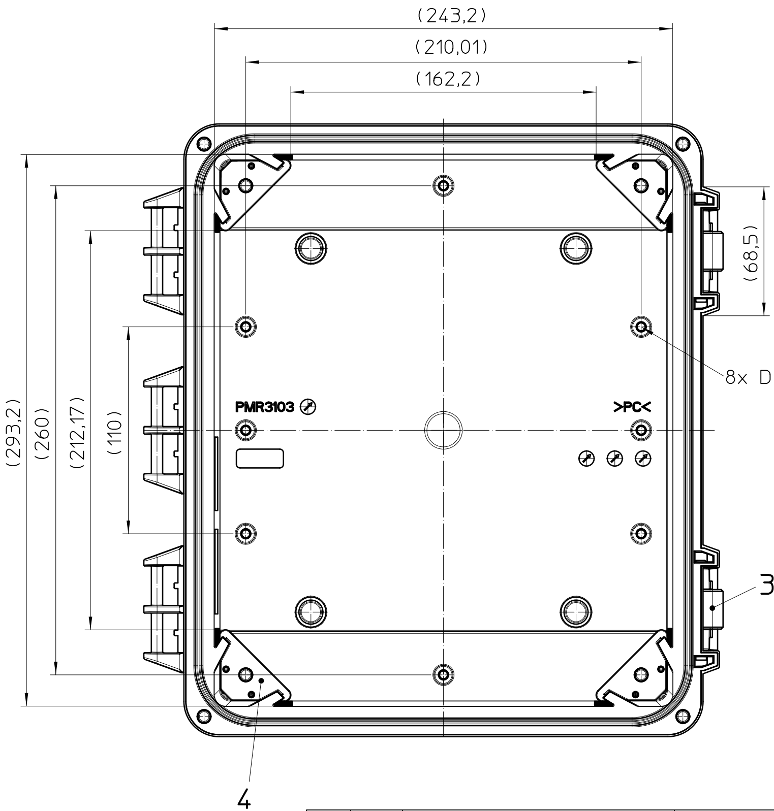
Front view without cover
