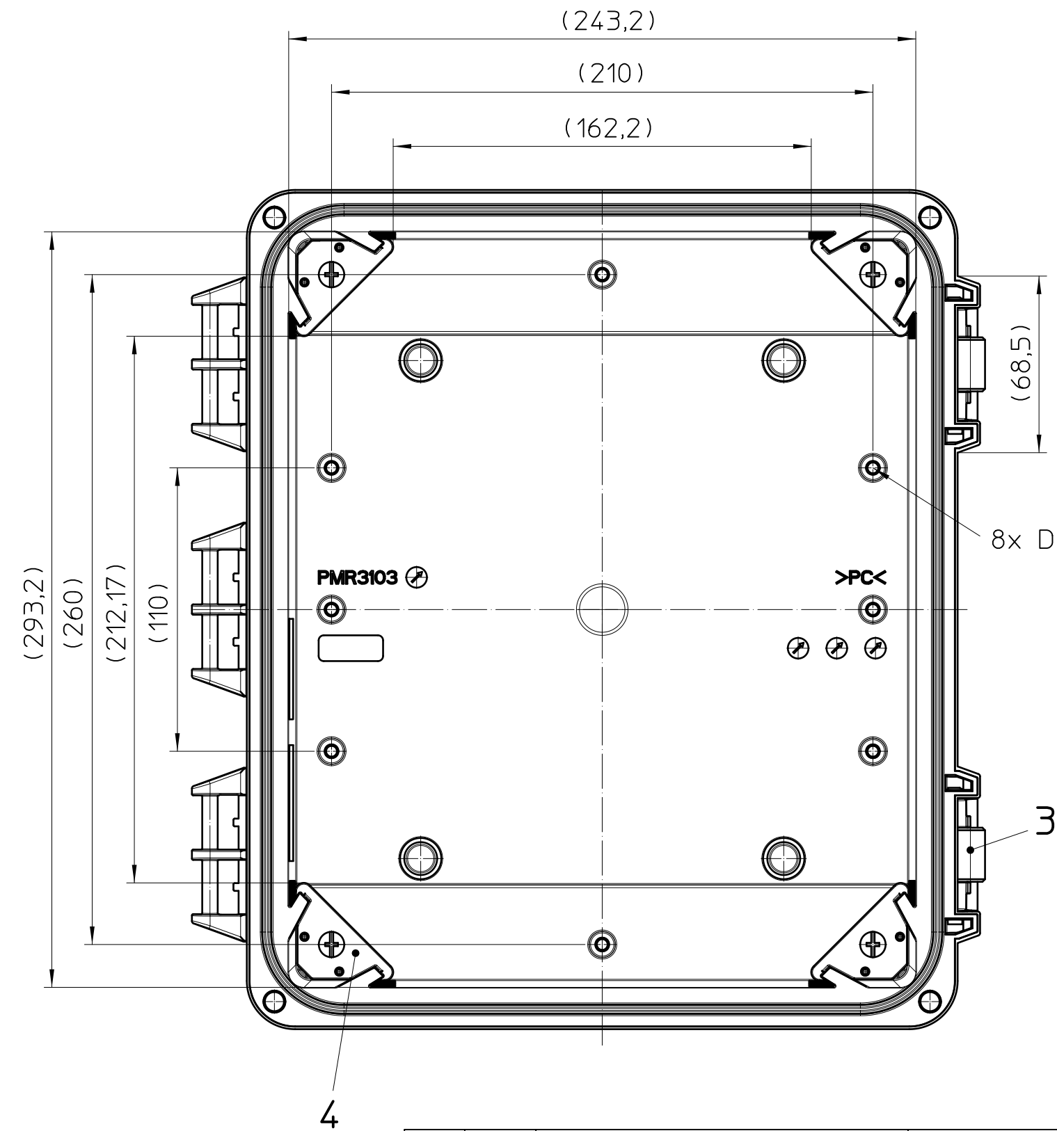
Front view without cover
