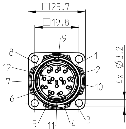
socket face female
